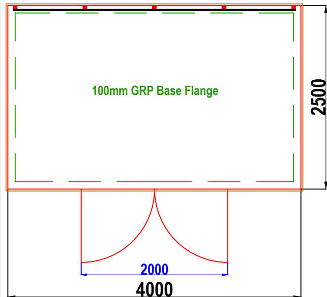
W21 WALK-IN GRP ENCLOSURE PLAN VIEW
