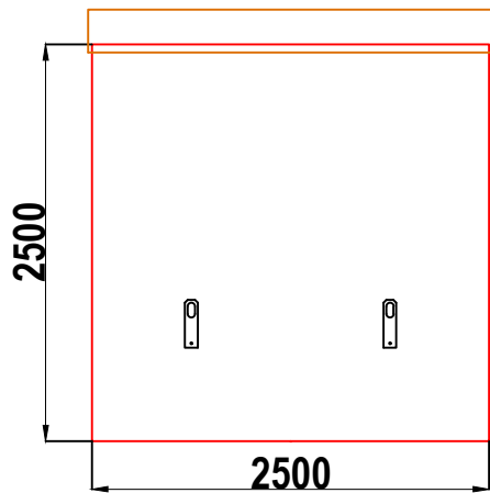
W21 WALK-IN GRP ENCLOSURE RIGHT HAND SIDE WALL ELEVATION WALL 3
