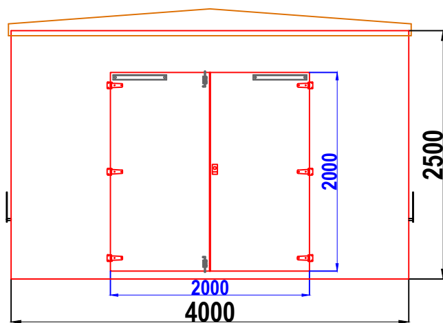
W21 WALK-IN GRP ENCLOSURE FRONT WALL ELEVATION WALL 1
