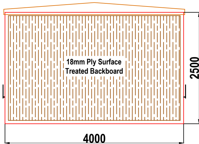
W21 WALK-IN GRP ENCLOSURE REAR WALL ELEVATION WALL 4
